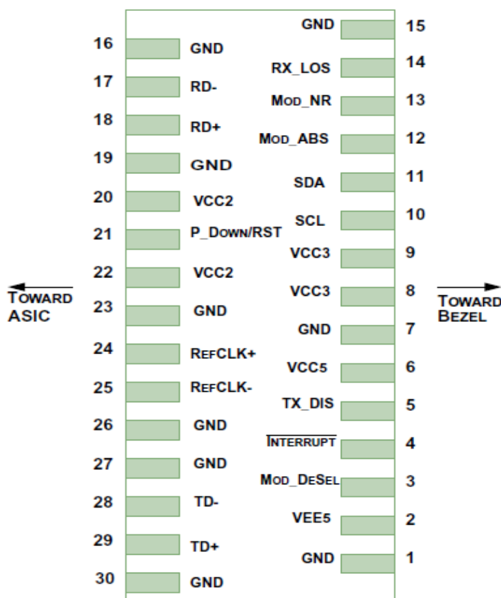
Diagram of Host Board Connector Block Pin Numbers and Name (Top View)
